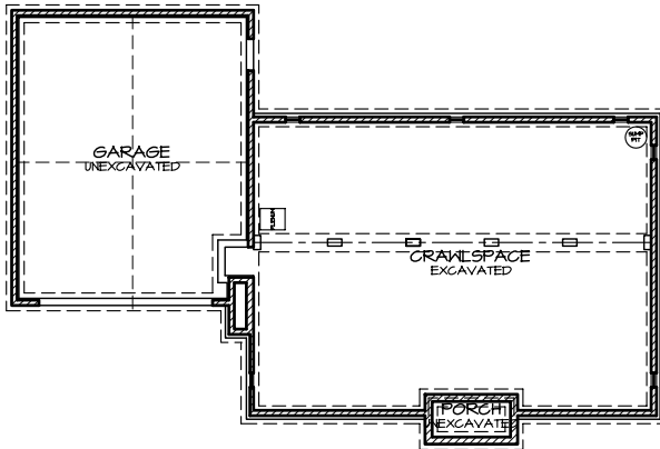
1 FOUNDATION PLAN A-2
