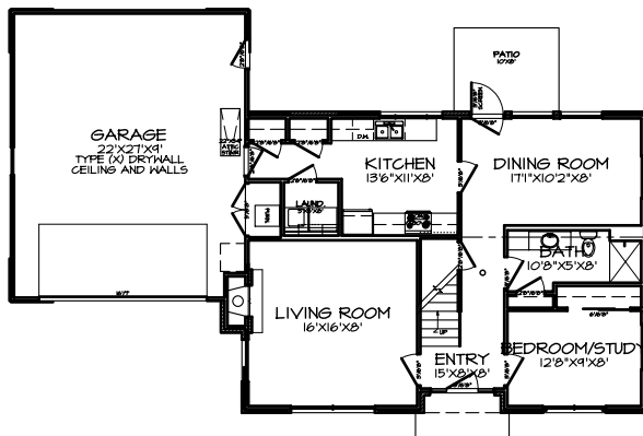
1 FIRST FLOOR PLAN A-3
